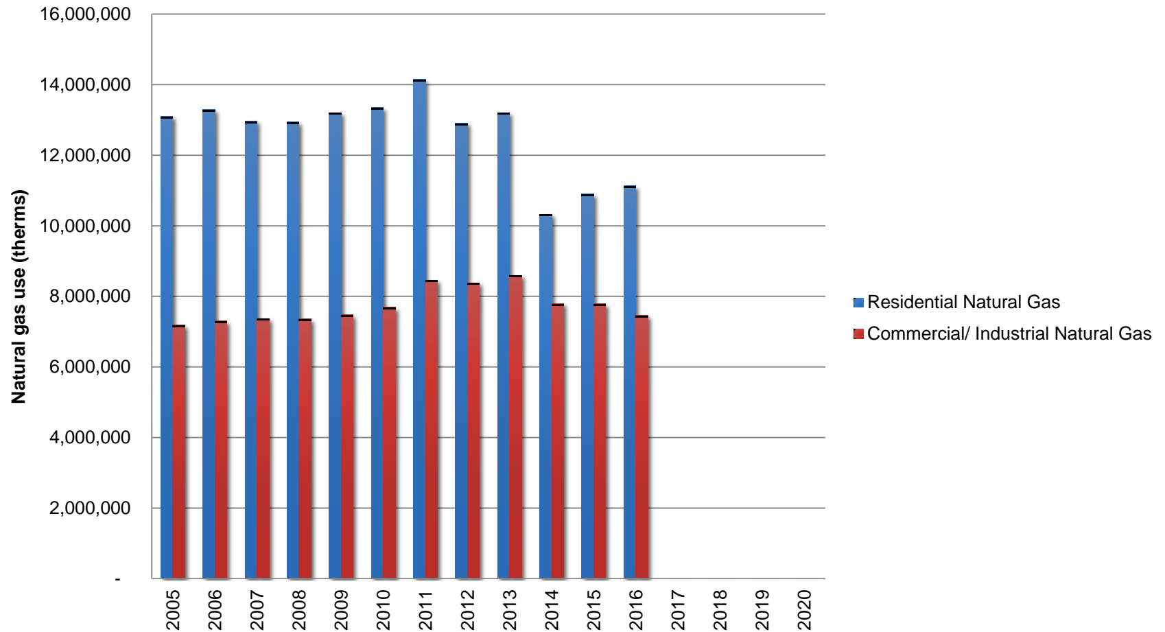
Annual Natural Gas use by Sector
